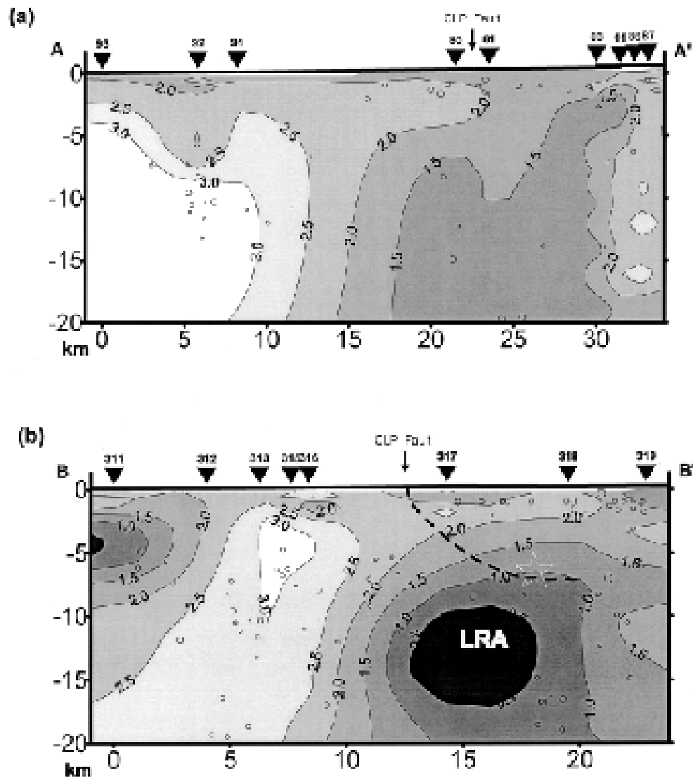
Fig. 3. Goelectric sections along profile AA' (a) and profile BB' (b) are indicated as shown in Fig. 1. The inverted triangles on the surface topography indicate the sounding points. Resistivities, in \log_{10} (resistivity) ohm-m, are contoured with values the lower the darker. The asterisk indicates the epicenter of the 1999 Chi-Chi earthquake in Taiwan, and the aftershocks with magnitude between 1 and 7 are indicated by open circles. The most significant feature in (b) is the existence of a distinct low resistivity anomaly (LRA) beneath the hypocenter of the Chi-Chi earthquake which was caused by fluids. Most of the large aftershocks occurred above the LRA and east of the CLP fault.
