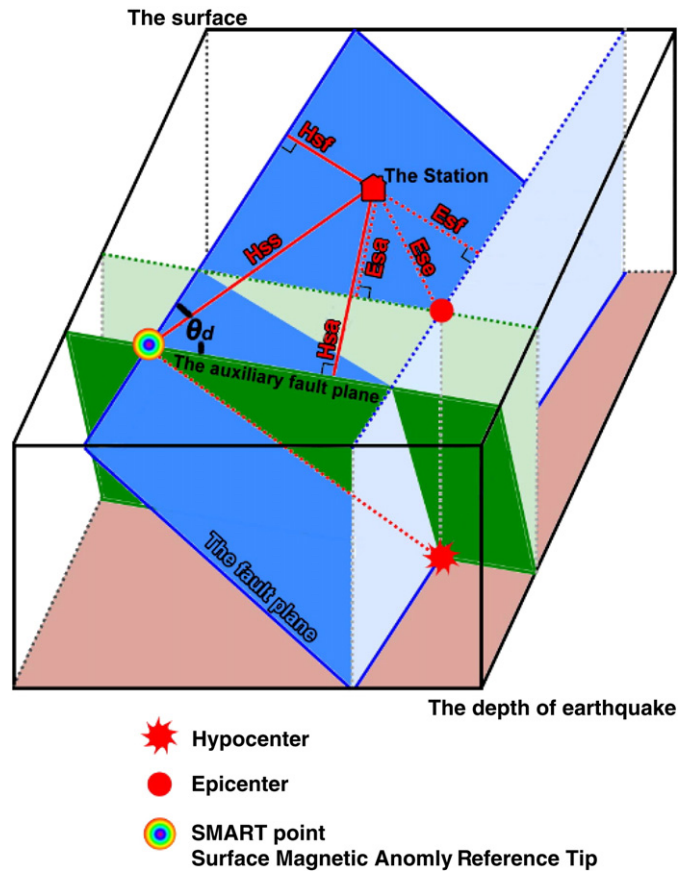
Fig. 3. The planned distribution of the two planes during an earthquake. The dashed line indicates the intersection of the fault and auxiliary fault planes; the hypocenter (red sun) and SMART (rainbow circle) point indicate the depth of the earthquake and the intersection on the line drawn through the surface, respectively. The red circle denotes the epicenter on the surface. Notably, regarding to the fault system, the anomalies are related with the distance from the stations to the fault line on the surface (Hsf). Ese, Esf and Esa are correlated to determine the position in the epicenter system and Hss, Hsf and Hsa denote the three different distances from the station of the two planes in the hybrid system. An angle, \theta_d , is determined between the fault and auxiliary fault lines on the surface.
